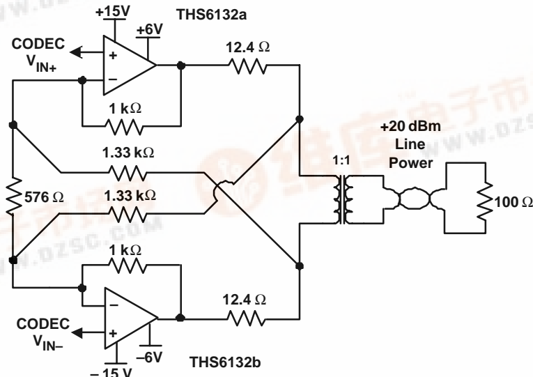
Typical ADSL CO Line Driver Circuit Utilizing Active Impedance Supporting A 6.3 Crest Factor
