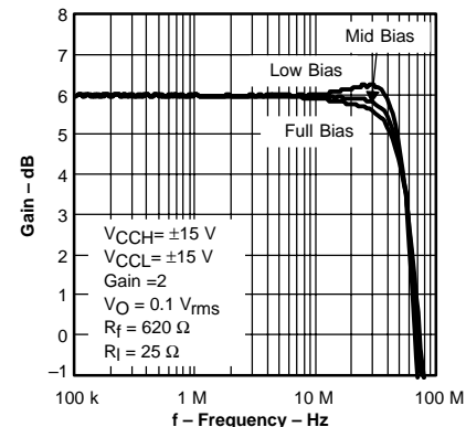
SMALL SIGNAL BANDWIDTH vs FREQUENCY
