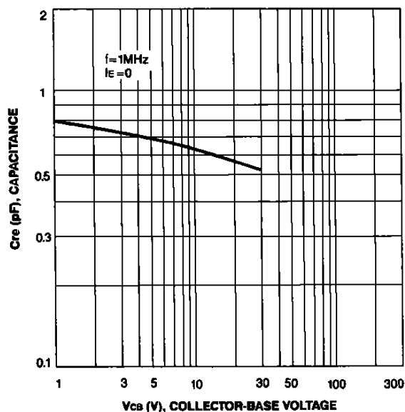
REVERSE CAPACITANCE
