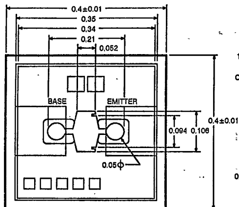
NE02100 (CHIP) (Chip Thickness: 140 \mu m)
