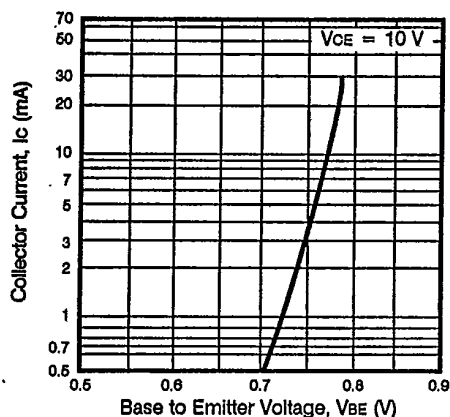
VOLTAGE CURRENT CHARACTERISTICS
