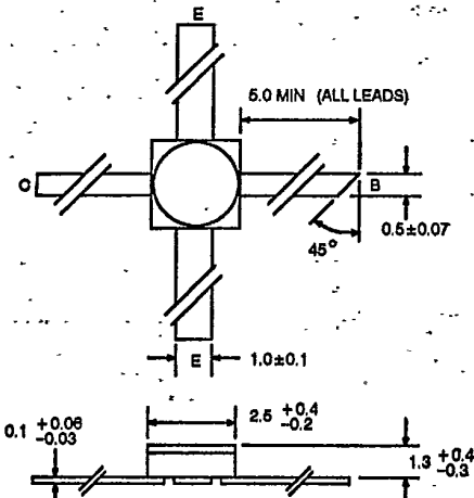
OUTLINE 07
