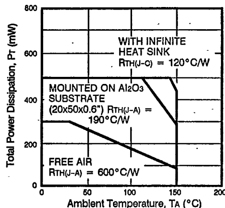
NE02135 DC POWER DERATING CURVES
