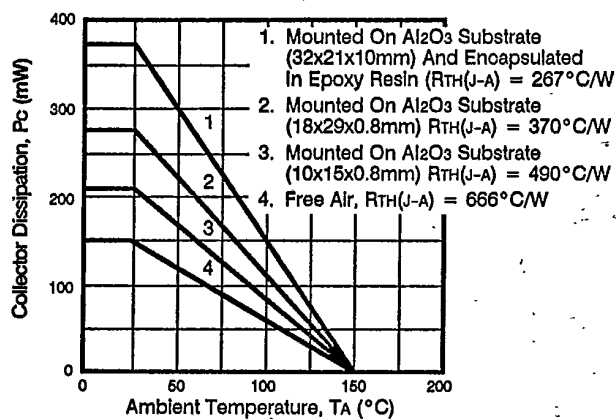
NE02133 DC POWER DERATING CURVES
