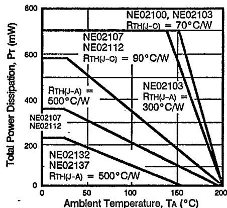
NE02100, NE02103, NE02107, NE02112, NE02132, NE02137 DC POWER DERATING CURVES
