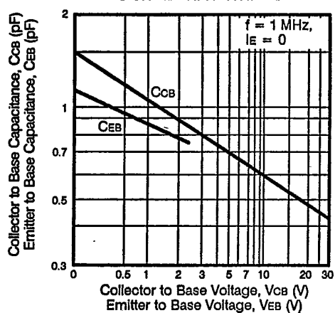
DEVICE CAPACITANCE
