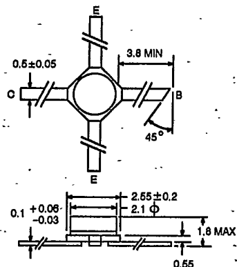
OUTLINE 35 (MICRO-X)
