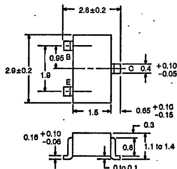
OUTLINE 33 (SOT-23)
