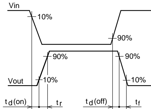
Switching Time Test Circuit Waveform
