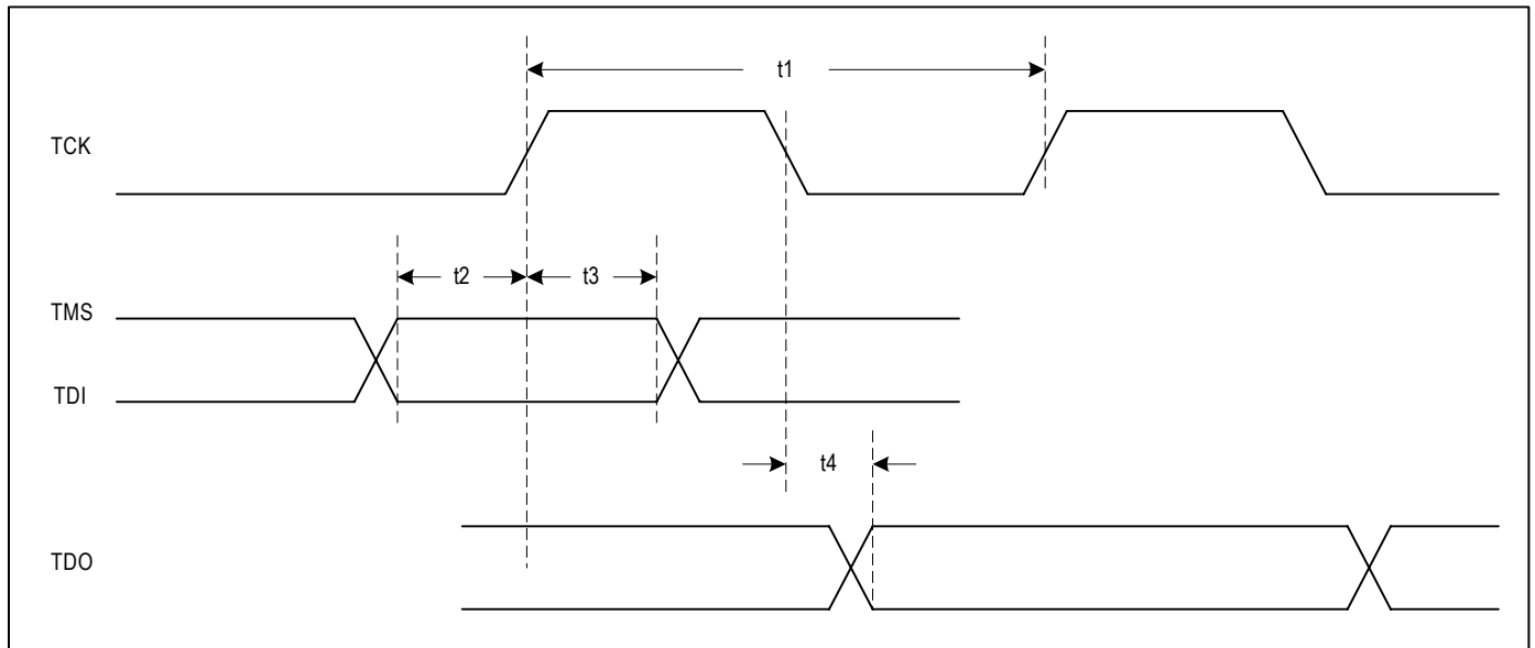
Figure-29 JTAG Interface Timing
