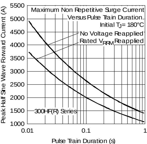
Fig. 6 - Maximum Non-Repetitive Surge Current
