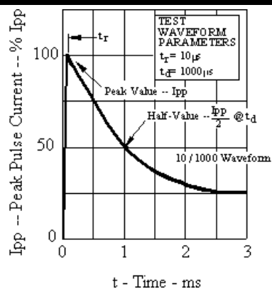
FIGURE 2 Pulse Wave Form
