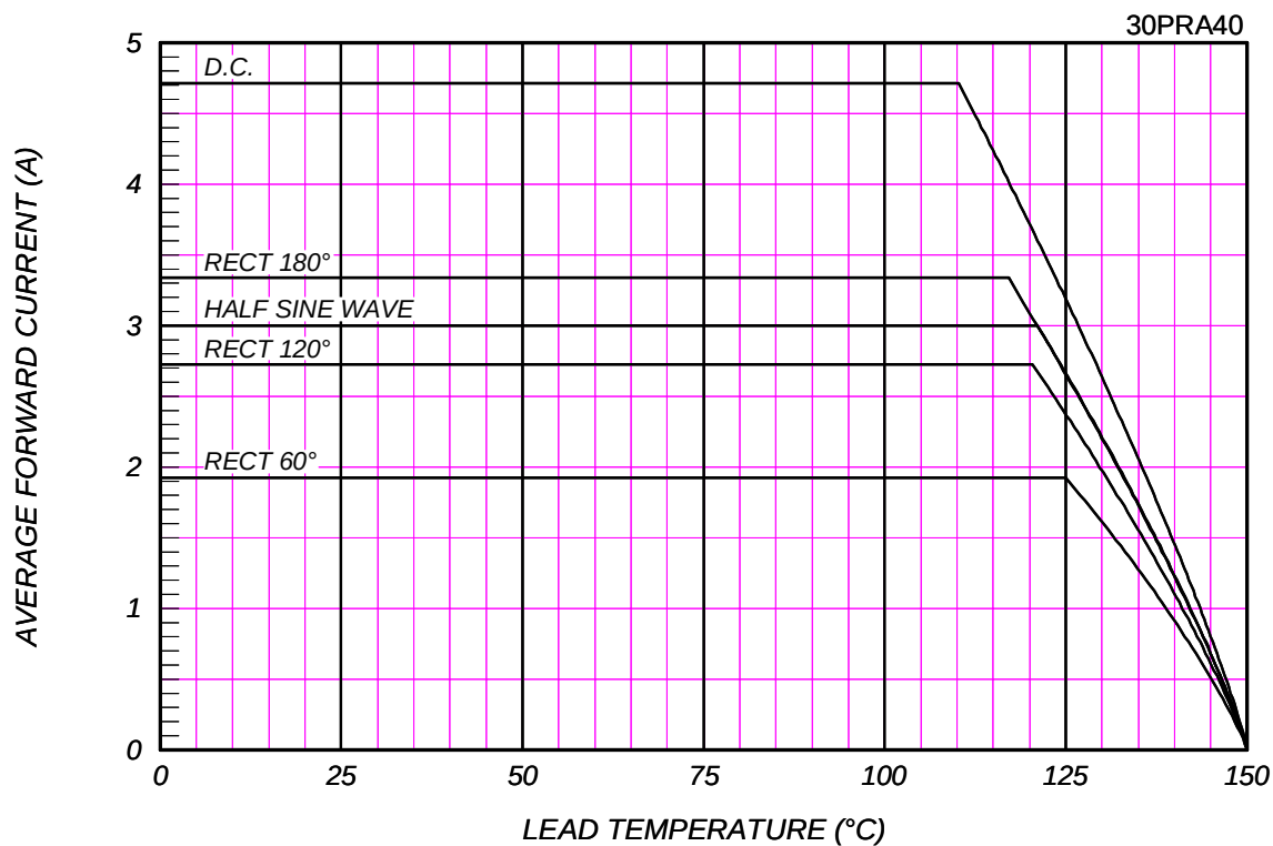
AVERAGE FORWARD CURRENT VS. LEAD TEMPERATURE
