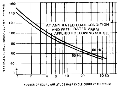
Fig. 5 - Maximum Non-Repetitive Surge Current
