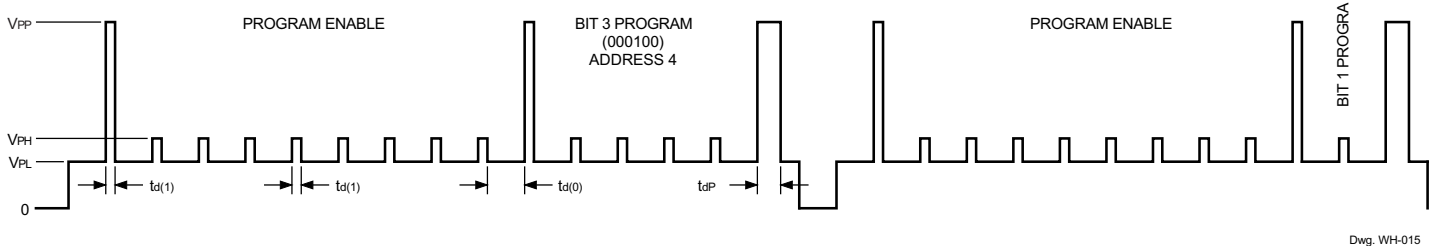
Figure 3 — Set-point programming
