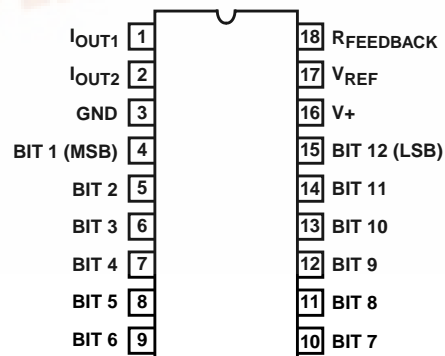
AD7521, AD7531 (PDIP) TOP VIEW
