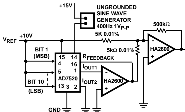
FIGURE 3. POWER SUPPLY REJECTION
