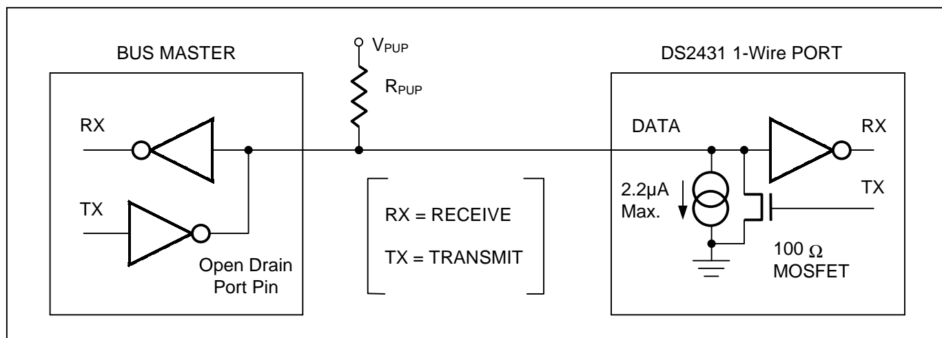
Figure 8. Hardware Configuration
