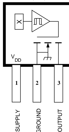
Package Designator 'UA' Pinning (SIP)
