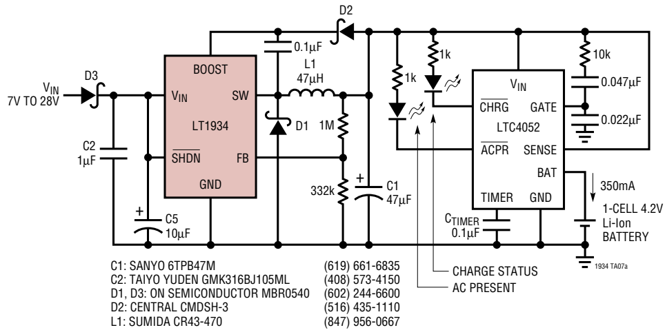
Standalone 350mA Li-Ion Battery Charger
