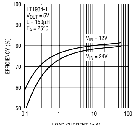
LT1934-1 Efficiency, V_{OUT} = 5\text{V}
