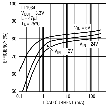
LT1934 Efficiency, V_{OUT} = 3.3\text{V}
