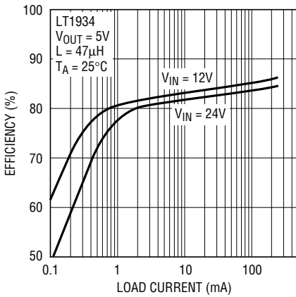
LT1934 Efficiency, V_{OUT} = 5\text{V}
