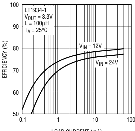
LT1934-1 Efficiency, V_{OUT} = 3.3\text{V}
