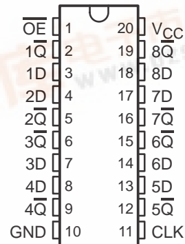
SN54AC534 . . . J OR W PACKAGE SN74AC534 . . . DB, DW, N, OR PW PACKAGE (TOP VIEW)
