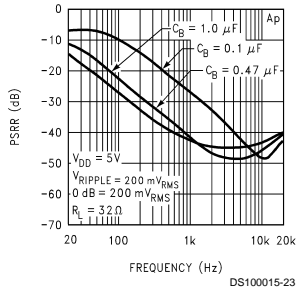
Power Supply Rejection Ratio Line Out/HP Amplifiers
