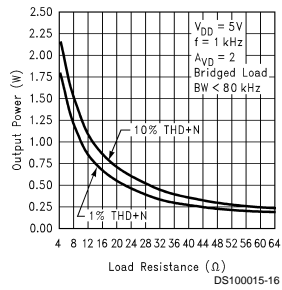
Output Power vs Load Resistance Bridged Power Amp
