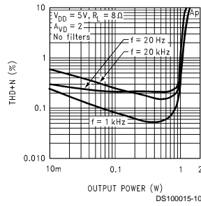
THD+N vs Output Power Bridged Power Amp
