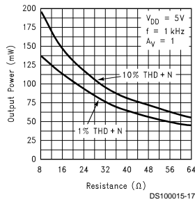
Output Power vs Load Resistance Line Out/HP Amplifiers
