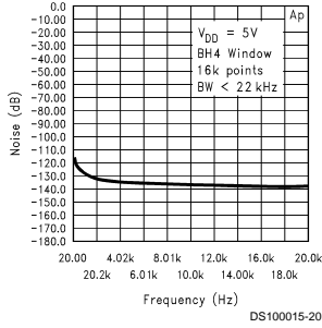
Noise Floor Line Out/HP Amp
