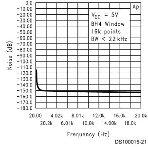
Noise Floor Mic Preamp
