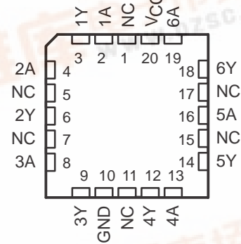
SN54ALS34, SN54AS34 . . . FK PACKAGE (TOP VIEW)
