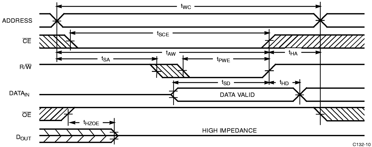
Write Cycle No. 2 (R/W Three-States Data I/Os-Either Port) [15, 24]
