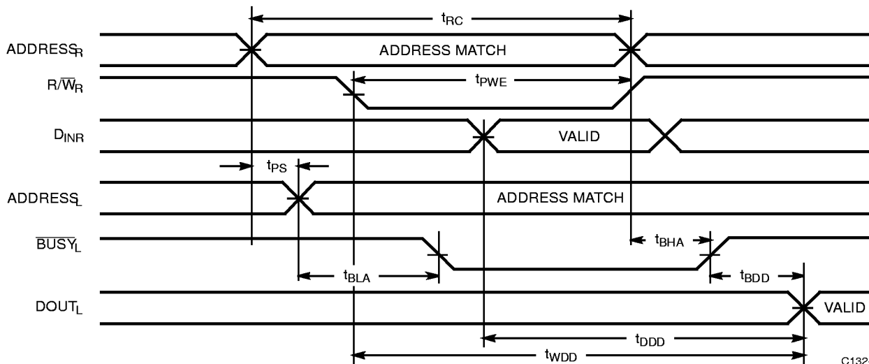
Read Cycle No. 3 (Read with BUSY Master: CY7C132 and CY7C136)
