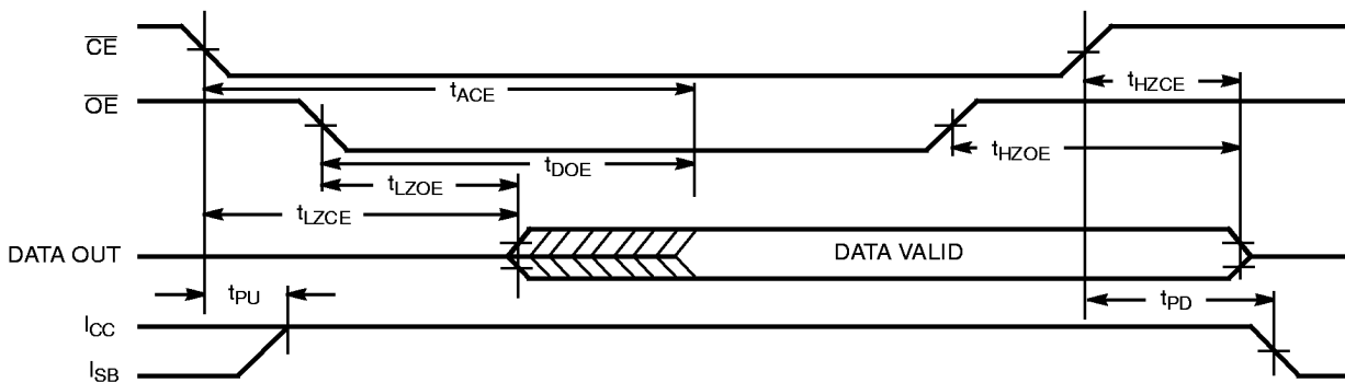
Read Cycle No. 2 (Either Port- \overline{CE}/\overline{OE} ) [20, 22]
