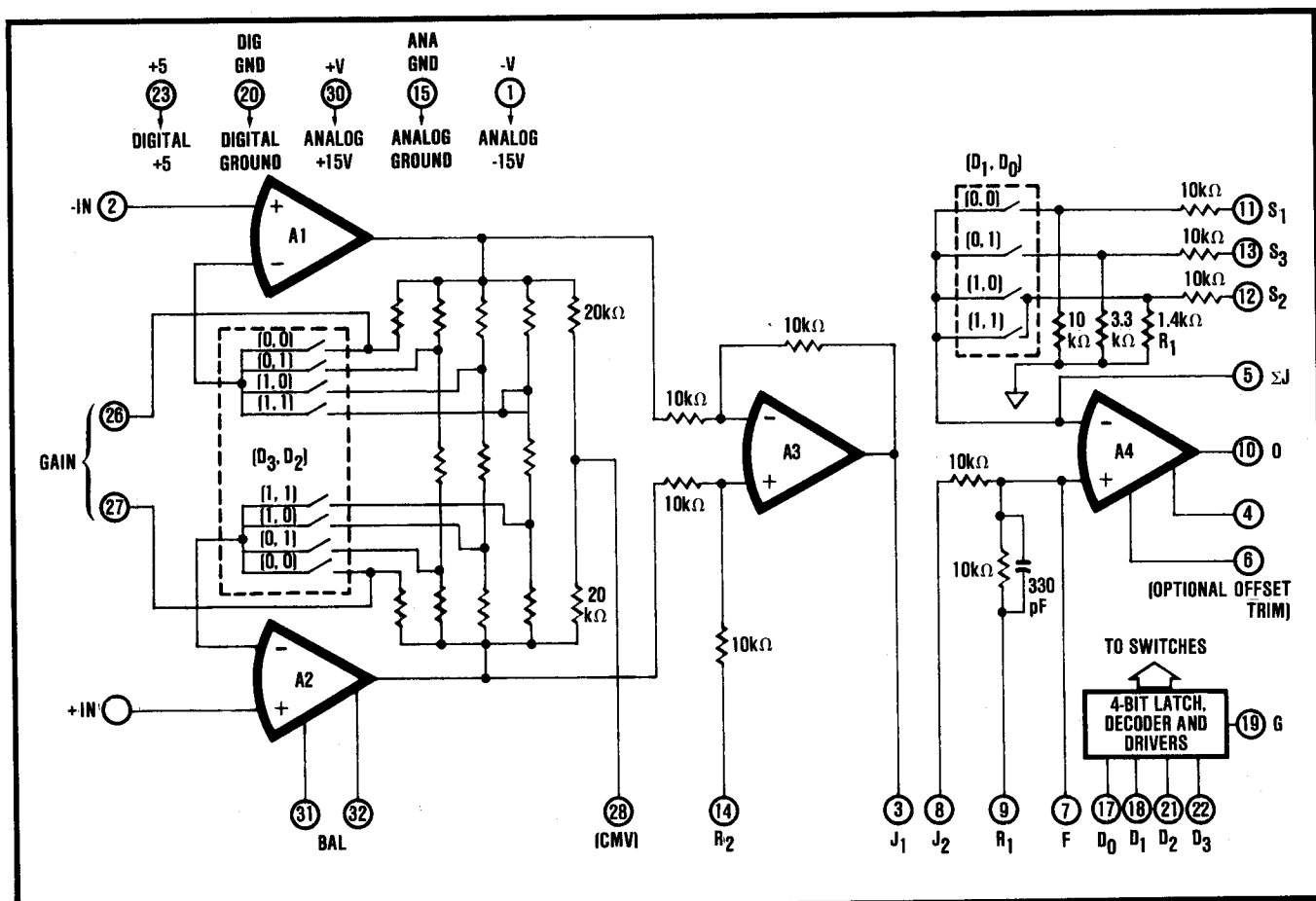
FIGURE 1. Simplified Schematic.
