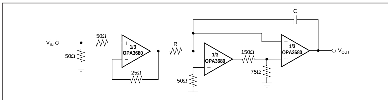
FIGURE 7. Wideband Integrator.
