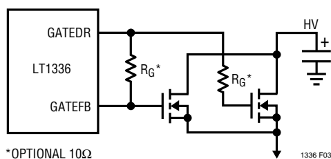
Figure 3. Paralleling MOSFETs
