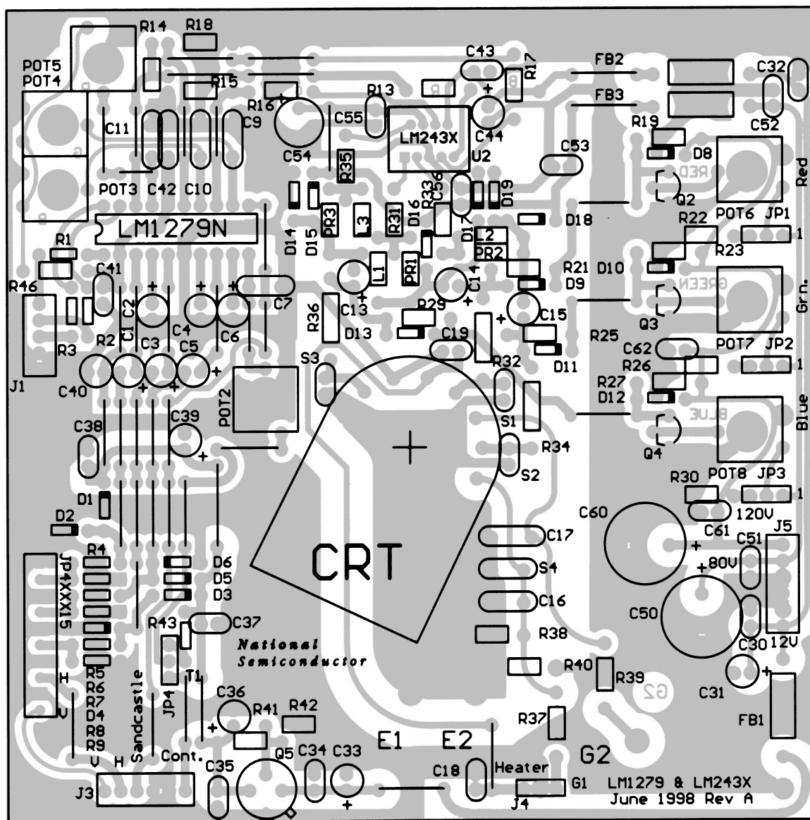
FIGURE 12. LM1279/243X Demo Board Layout
