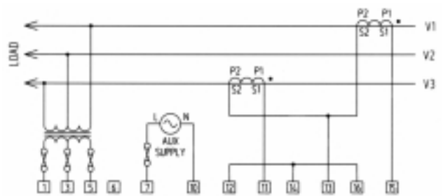
3-Phase 3-Wire Using Potential Transformers
