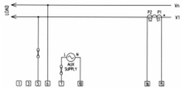
Single Phase
