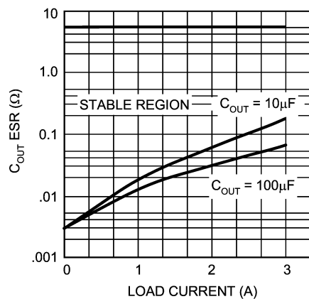
20069731 Minimum ESR vs Output Load Current
