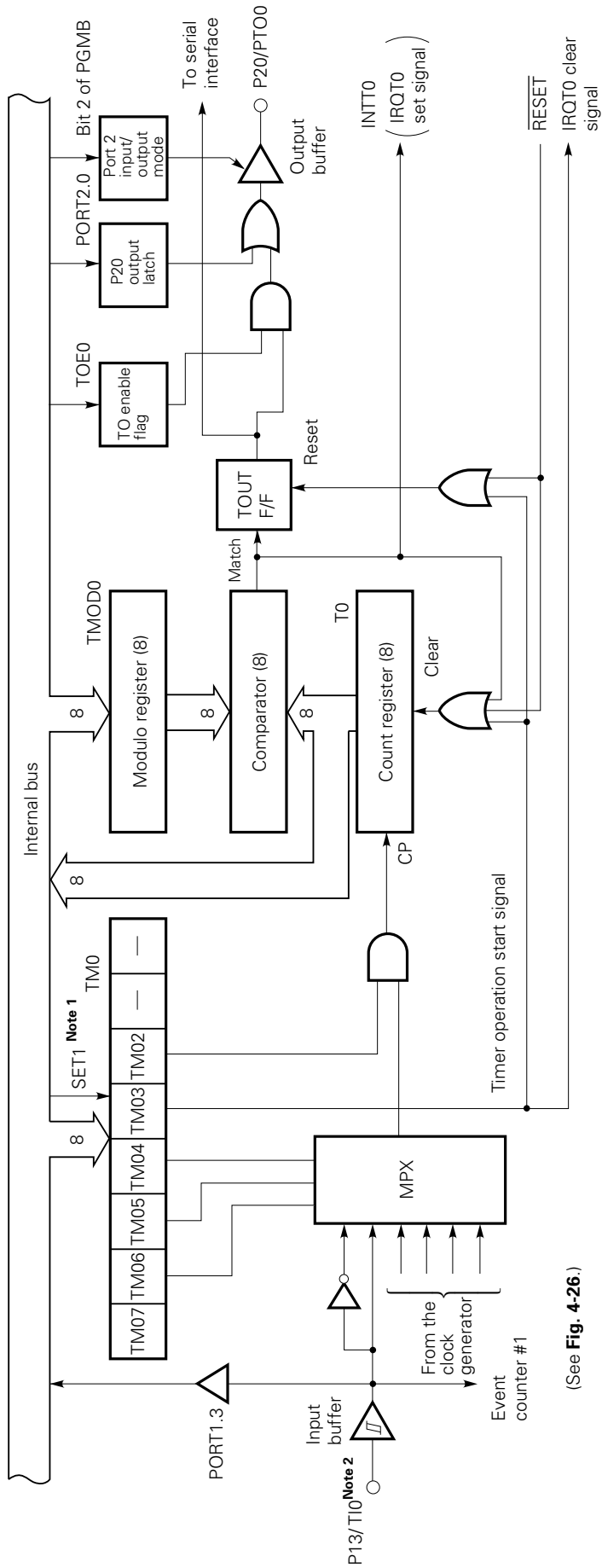
Fig. 4-25 Block Diagram of the Timer/Event Counter
