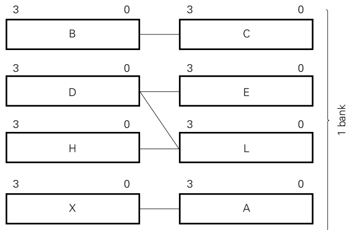
Fig. 3-6 Register Pair Format
