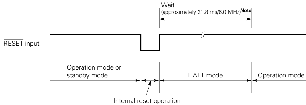
Fig. 7-2 Reset Operation by \overline{\text{RESET}} Input
