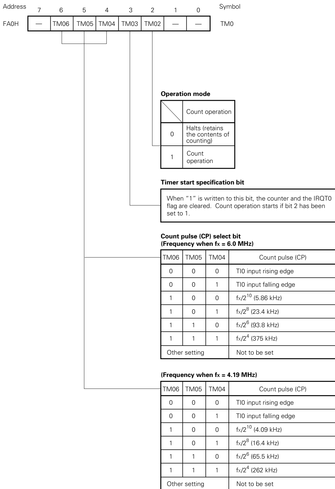
Fig. 4-27 Format of the Timer/Event Counter Mode Register
