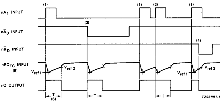
Fig.6 Timing diagram.
