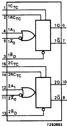
Fig.4 Functional diagram.
