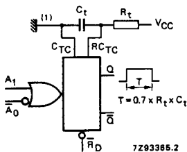
Fig.5 Connection of the external timing components R t and C t .
