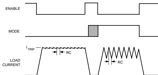
Dwg. WP-015-1
