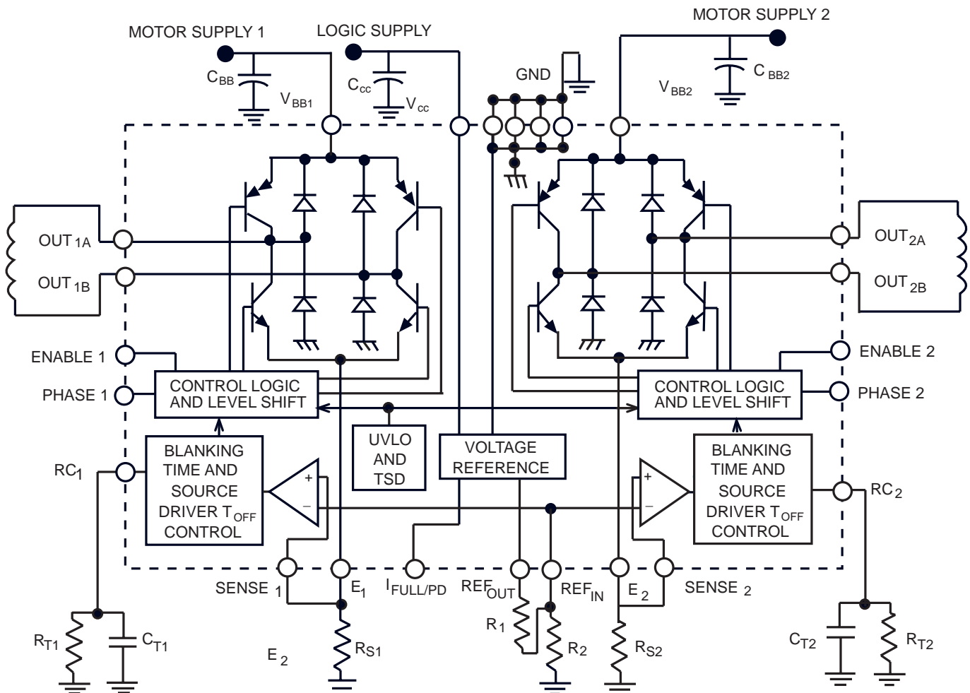
FUNCTIONAL BLOCK DIAGRAM AND TYPICAL BIPOLAR STEPPER MOTOR APPLICATION
