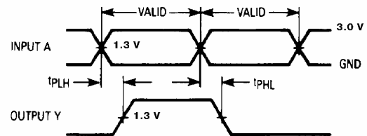
Figure 2. Switching Waveforms
