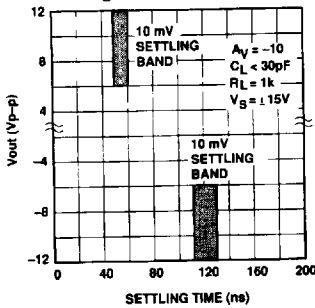
Settling Time
