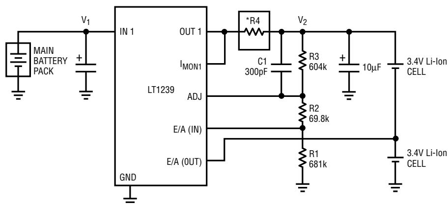
Figure 5. Adding a Protection Resistor for Lithium-Ion Charger
