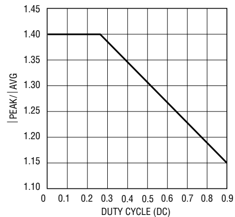
Figure 6. Maximum Ripple Current (Normalized) vs Duty Cycle for Average Current Limit
