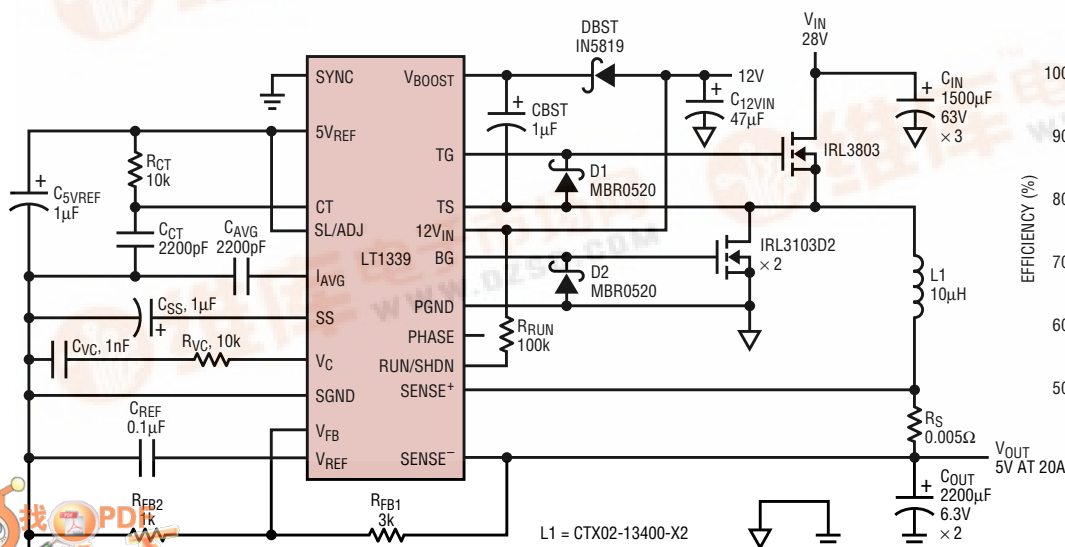
28V to 5V 20A Buck Converter
