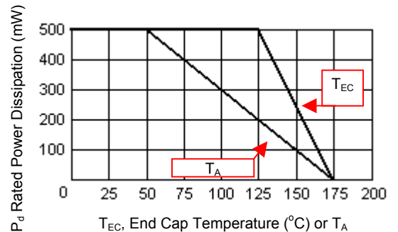
FIGURE 2 Power Derating Curve T EC , End Cap Temperature (°C) or T A Ambient temperature on FR4 PC board
