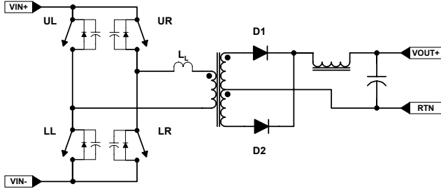
FIGURE 10. IDEALIZED FULL-BRIDGE
