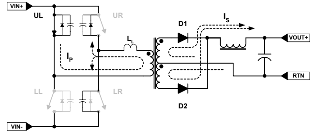
FIGURE 12. UL - UR FREE-WHEELING PERIOD
