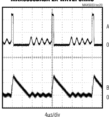
MAX5033BASA LX WAVEFORMS
