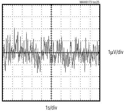
0.1Hz TO 10Hz OUTPUT NOISE ( V_{OUT} = 2.5V )
