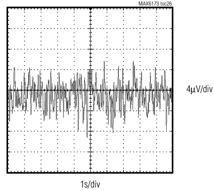
0.1Hz TO 10Hz OUTPUT NOISE ( V_{OUT} = 10V )
