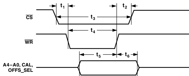
Figure 1. Parallel Write (SHA Mode Only)
