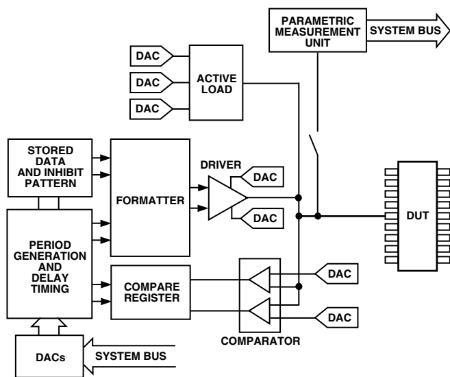
Figure 24. AD5532 in an ATE System
