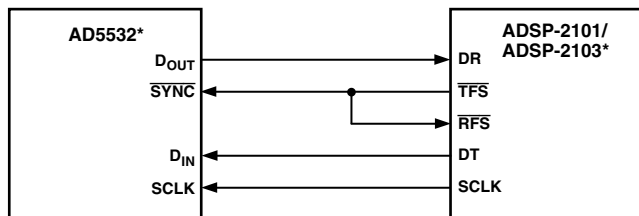
Figure 20. AD5532 to ADSP-2101/ADSP-2103 Interface
