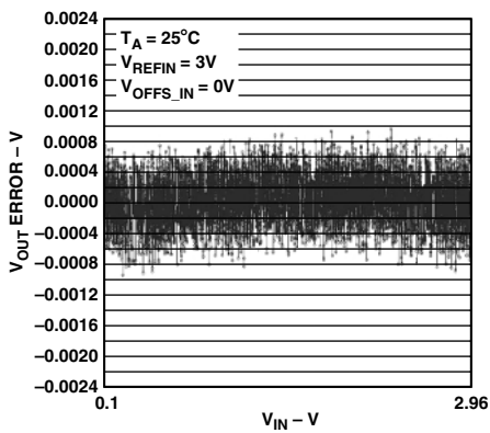
Figure 14. V_{IN} to V_{OUT} Accuracy After Offset and Gain Adjustment (SHA Mode)
