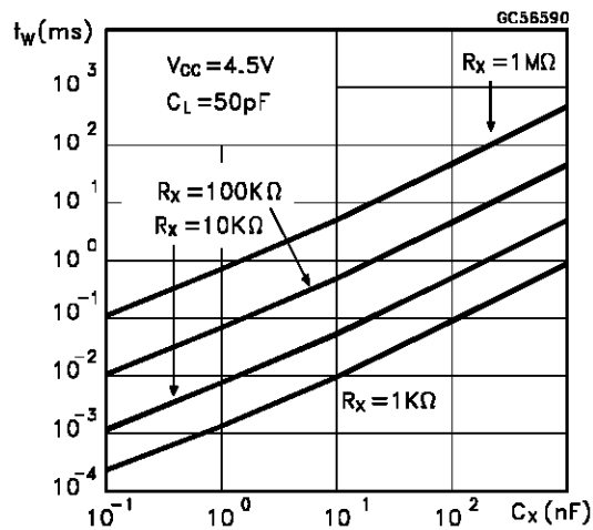
Output Pulse Width Characteristics (for HC123)
