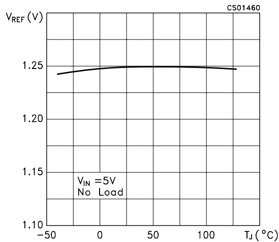
Figure 3 : Reference Voltage vs Temperature
