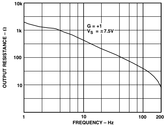
Figure 14. Output Resistance vs. Frequency, Disabled State
