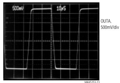
DYNAMIC RESPONSE
