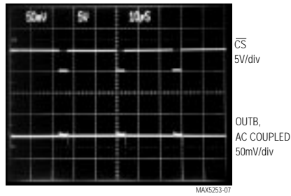
MAJOR-CARRY TRANSITION
