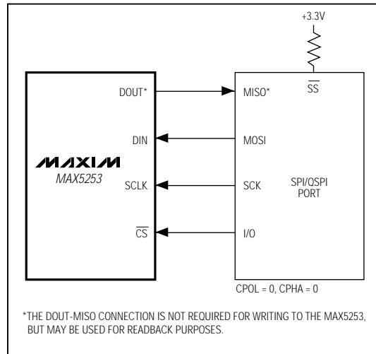
Figure 3. Connections for SPI/QSPI
