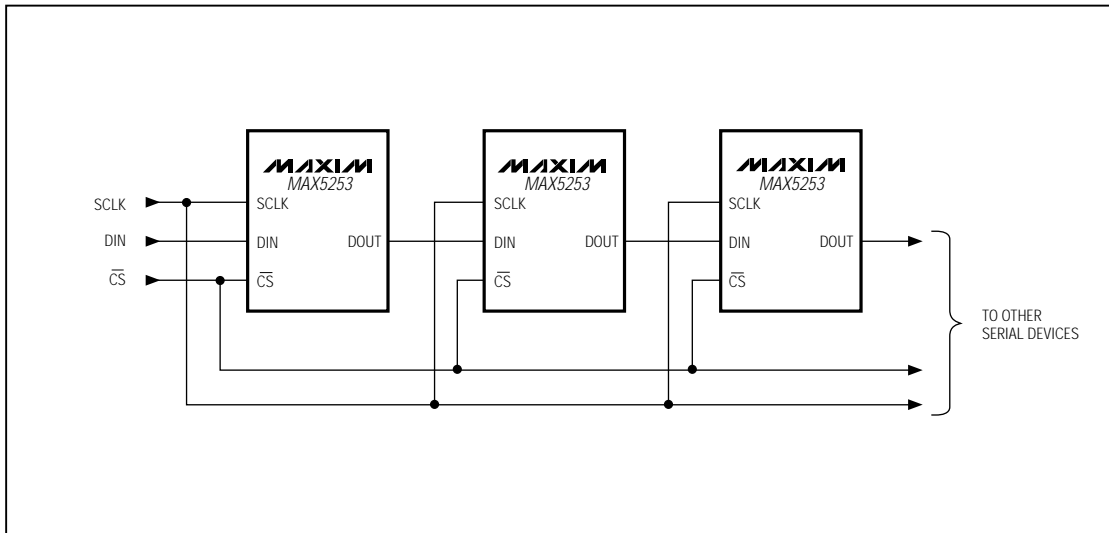
Figure 7. Daisy-Chaining MAX5253s
