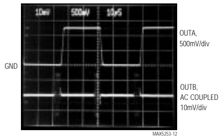
ANALOG CROSSTALK
