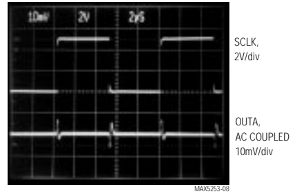
DIGITAL FEEDTHROUGH (SCLK = 100kHz)
