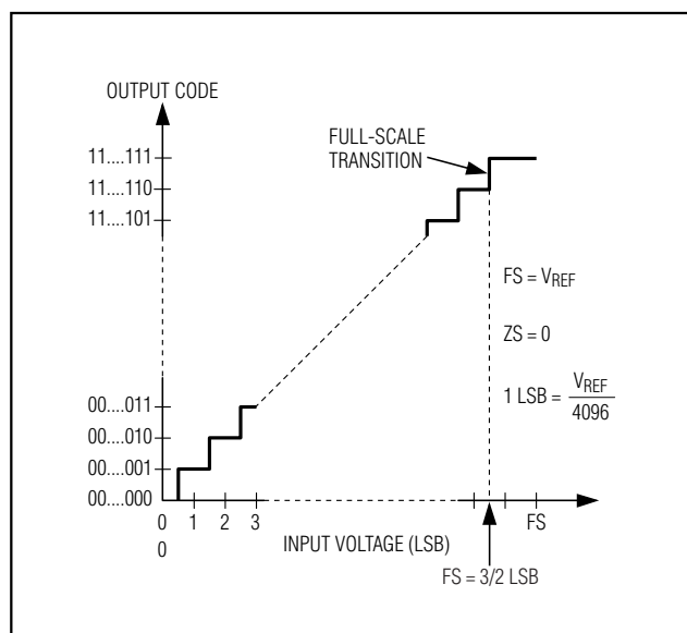
Figure 10. Unipolar Transfer Function, Full Scale (FS) = V REF
