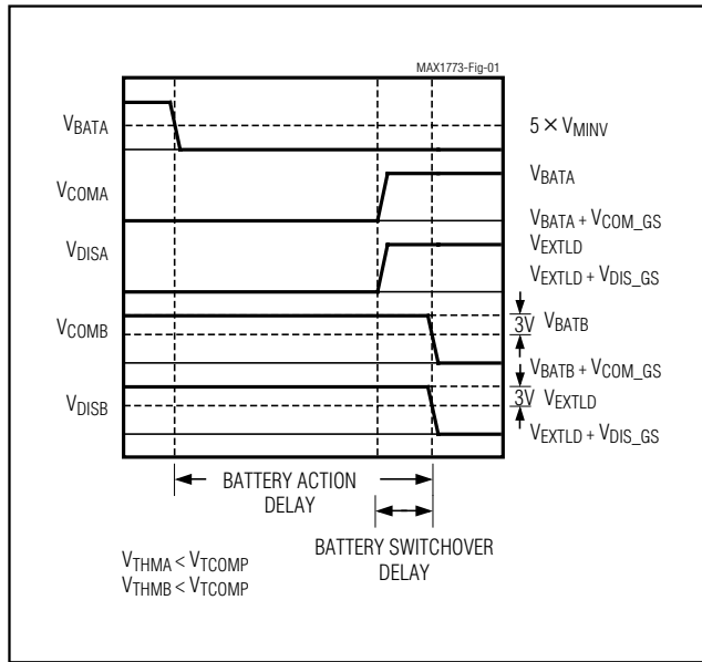
Figure 1. Battery Delay (Battery A to Battery B)
