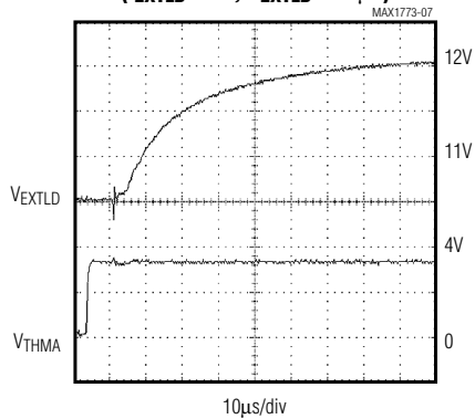
TRANSITION FROM BATTERY A TO BATTERY B (T COMP ) ( I_{\text{EXTLD}} = 4\text{A} , C_{\text{EXTLD}} = 66\mu\text{F} )
