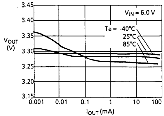
1.8 Output voltage ( V_{OUT} ) – Temperature
