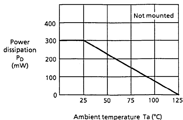
Figure 20 Power dissipation
