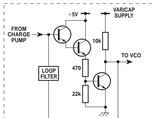
Fig. 6d Simple discrete amplifier
