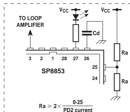
Fig. 6c Use of lock detect circuit with PD1
