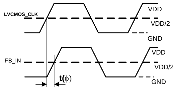
Figure 6. LVC MOS Propagation Delay t(\phi) , Static Phase Offset
