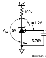
FIGURE 4. Thevenin Equivalent of Reference with 5V Output
