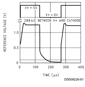
Reference Power-Up Time
