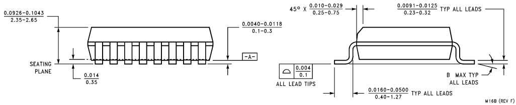
16-Lead Small Outline Package (WM) Order Number LM613IWM NS Package Number M16B
