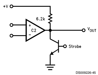
FIGURE 17. Basic Comparator with External Strobe DS009226-45
