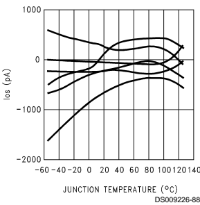
Input Offset Current vs Junction Temperature
