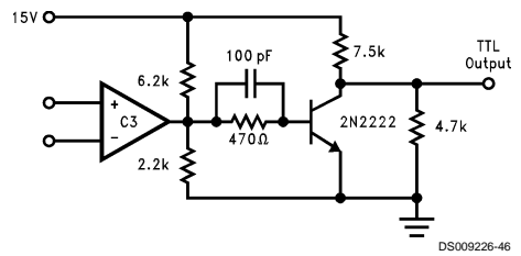
FIGURE 18. Wide-Input Range Comparator with TTL Output DS009226-46
