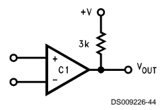
FIGURE 16. Basic Comparator DS009226-44
