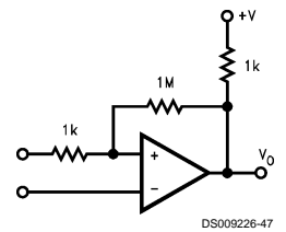
FIGURE 19. Comparator with Hysteresis ( \Delta V_H = +V(1k/1M) ) DS009226-47
