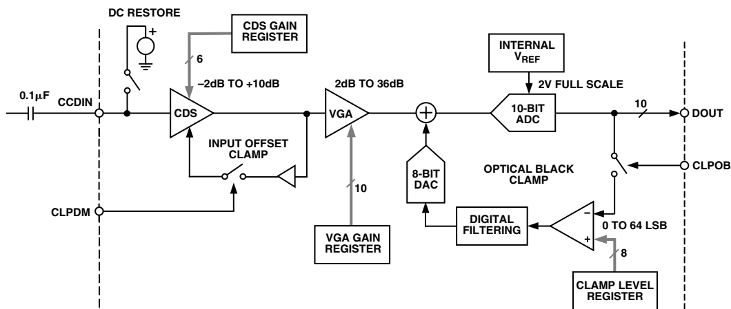
Figure 11. CCD-Mode Block Diagram
