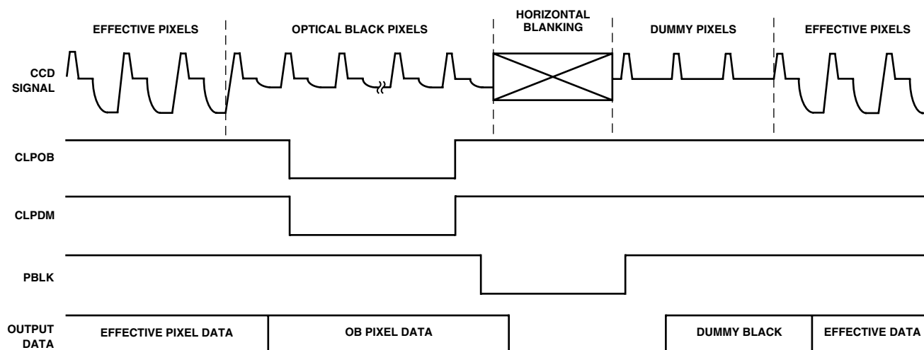
Figure 5. CCD-Mode Timing
