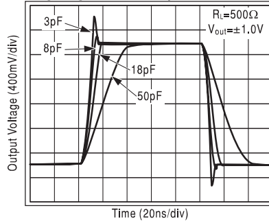
Settling Time vs. C_{comp}
