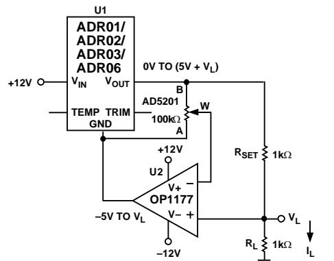
Figure 41. Programmable 0 to 5 mA Current Source
