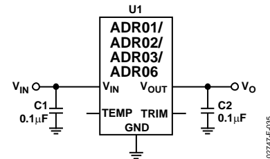
Figure 35. Basic Configuration
