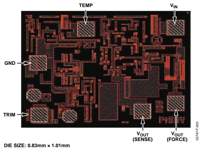
Figure 3. Die Layout
